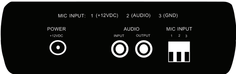
Rear Connections
